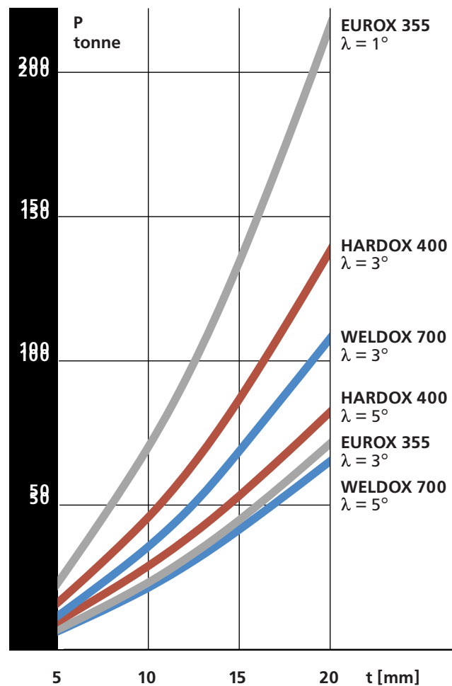
Fig. 3. Shearing force as a function of the thickness and rake angle λ
